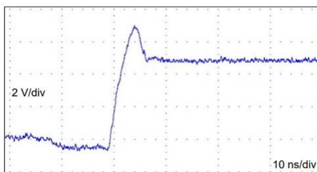
Figure 13. R_{SNB}=3.3\Omega , C_{SNB}=680\text{ pF}
