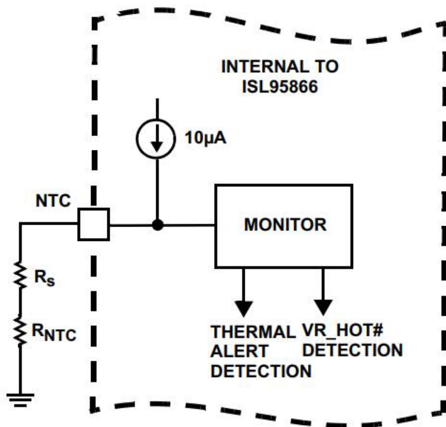
FIGURE 43. NTC CIRCUITRY
