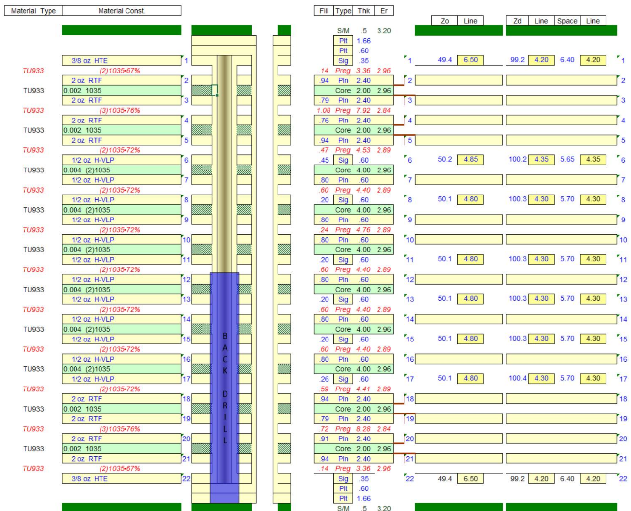
Figure 36: Wedge-100 TUC-933 PCB Stackup( Courtesy of ISU-Petasys)
