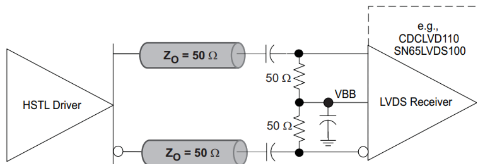
Figure 26. HSTL to LVDS
