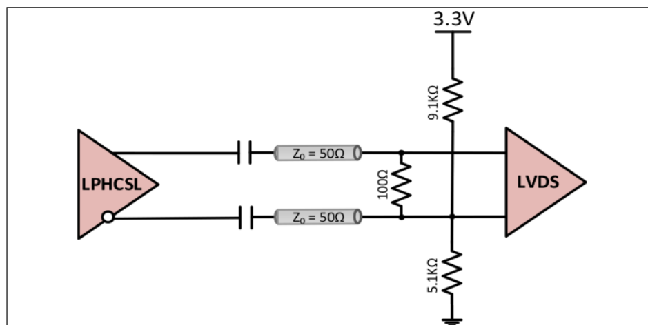
FIGURE 32: AC COUPLING LPHCSL TO LVDS.
