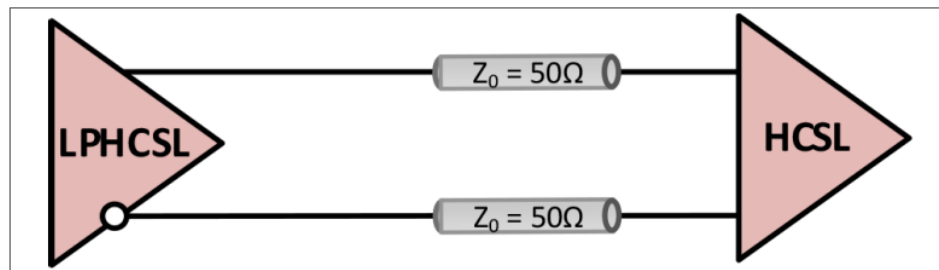
FIGURE 15: DC COUPLING LPHCSL TO HCSL.
