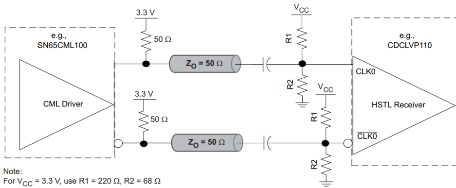
Figure 21. CML to HSTL
