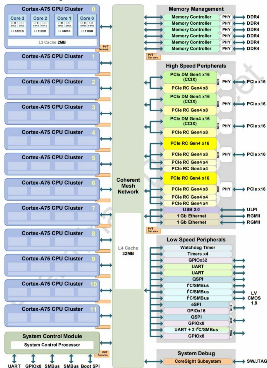
Figure 1-1 Block Diagram
