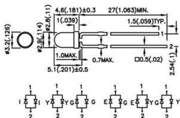
T-1 (3mm) Round
